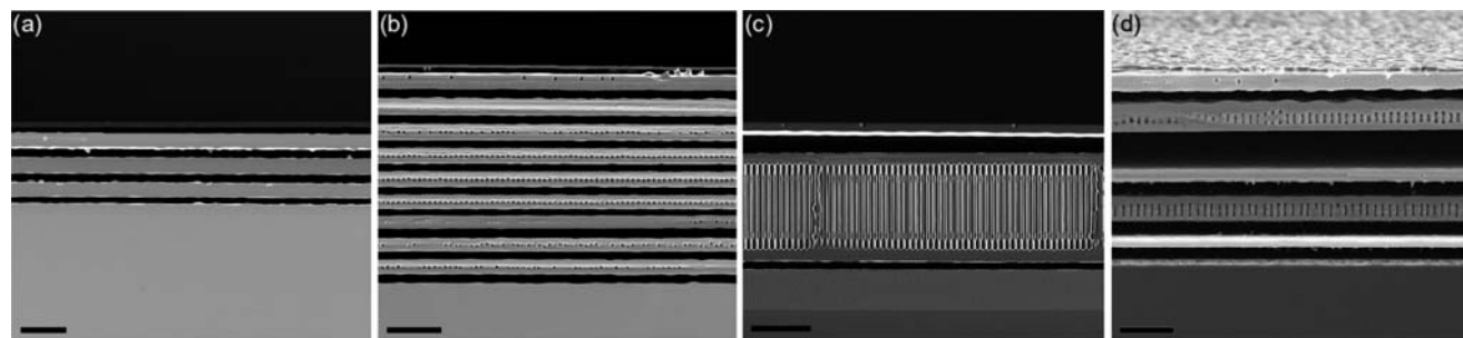
FIG. 5. SEM images of final layers' formation: (a) solid layers with 6.5 \mu\text{m} average thickness; (b) 10 layers with 5.9 \mu\text{m} average thickness with a row of pores inside; (c) thick layer formation (38 \mu\text{m} ) due to low-amplitude pore modulation; and (d) controlled thickness multilayer with alternate films of 4 and 8 \mu\text{m} thickness. Scale bars are 20 \mu\text{m} .
